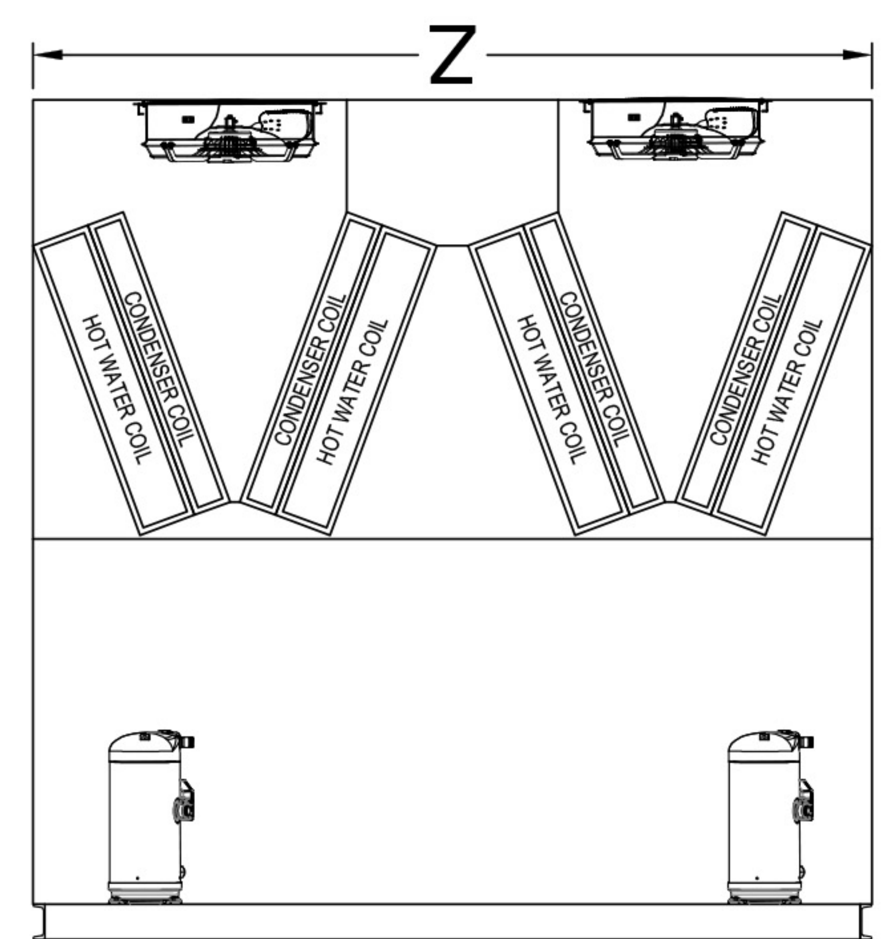
SIDE VIEW
