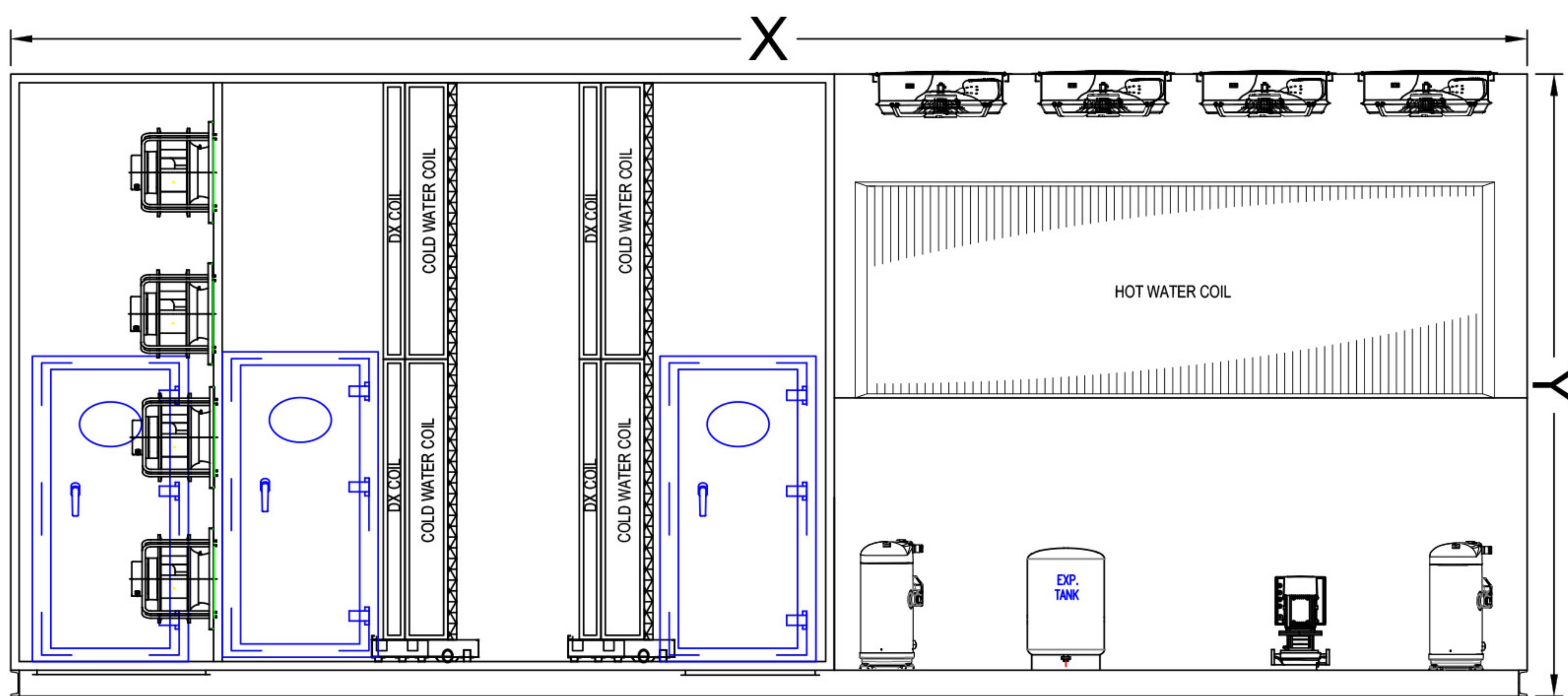
FRONT VIEW
